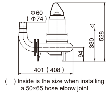
Y Hard Pipe Movable Installation
