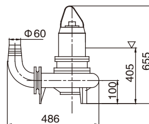
R Hose Movable Installation
