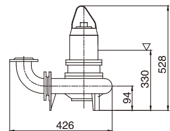
Y Hard Pipe Movable Installation
