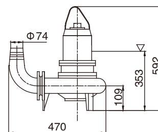
Y Hard Pipe Movable Installation
