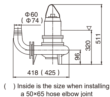
Y Hard Pipe Movable Installation
