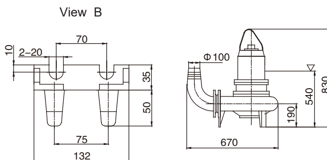
Y Hard Pipe Movable Installation
