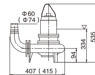
R Hose Movable Installation
