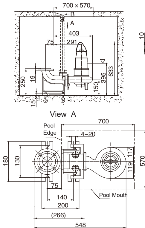
Z Automatic Coupling Installation
